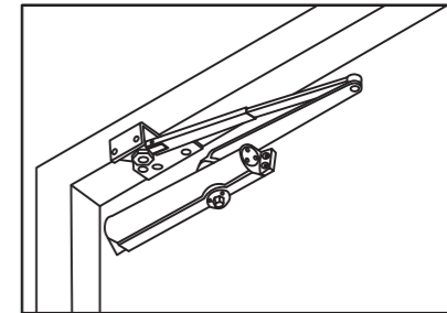
PARALLEL MOUNT (PUSH SIDE)
