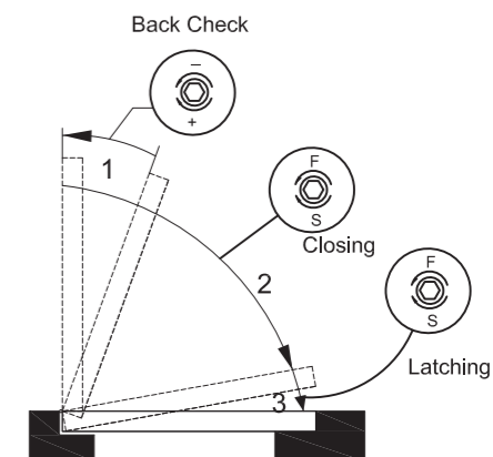
CONTROL RANGE
