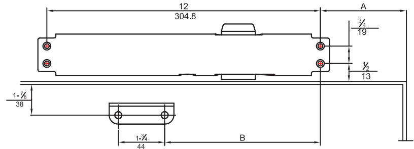
INSTALLATION DIMENSIONS
