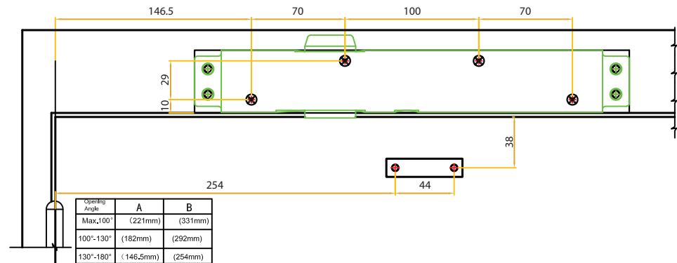
Top Jamb installation template with REG
