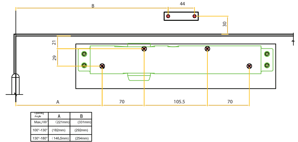
Regular installation template with REG
