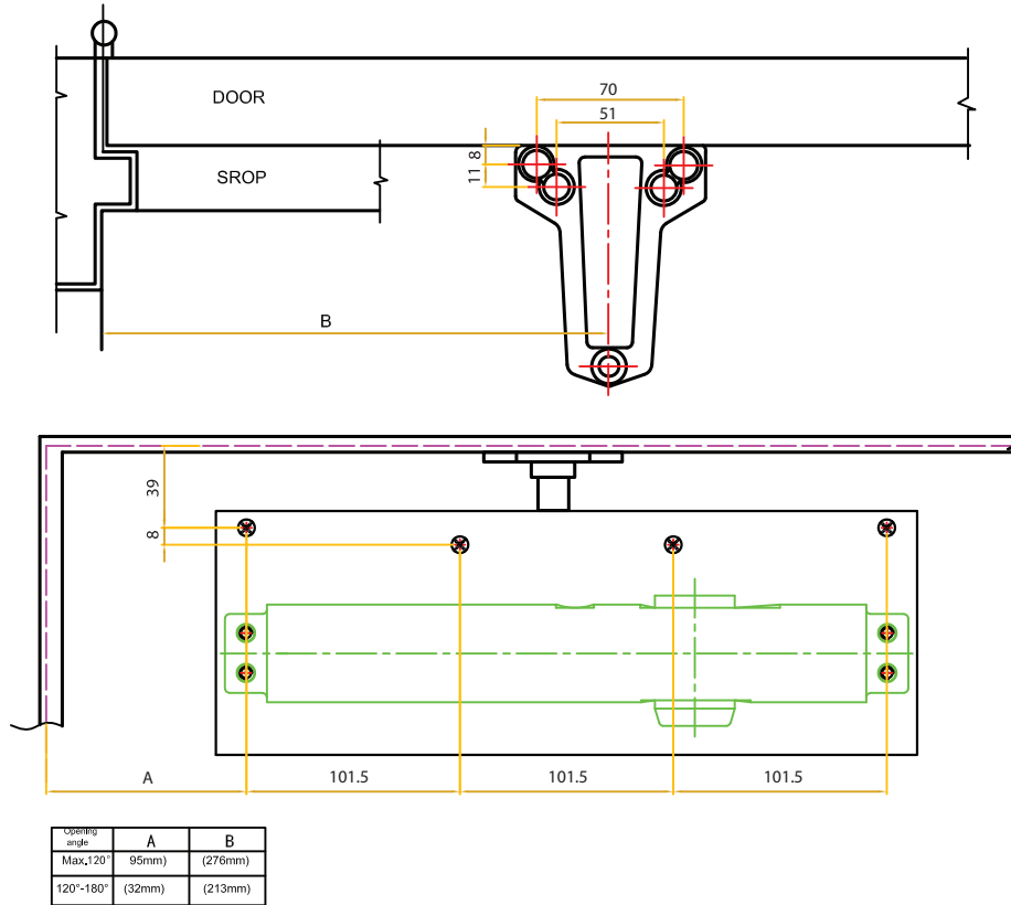
Parallel installation template with PA
