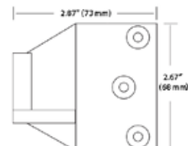
OED245-AL Overlapping Strike for Double Door Use in 5500/8500 Series
